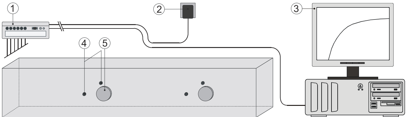
Figure 1 TRSYS01 consists of MCU02 Measurement and Control Unit (1), an adapter for power (2), 2 pairs of matched thermocouples (4), and 2 heat flux plates of type HFP01 (5). MCU02 measures and stores data. Readout is performed by connecting temporarily to a PC (3) (not included). Software for readout is included.
