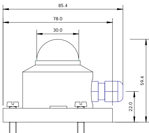
Figure 2 LP02 dimensions. Standard cable length is 5 m. Cable can be installed / replaced by the user.
