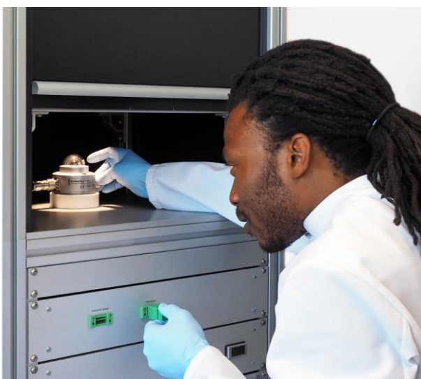
Figure 3 a typical calibration system at Hukseflux
