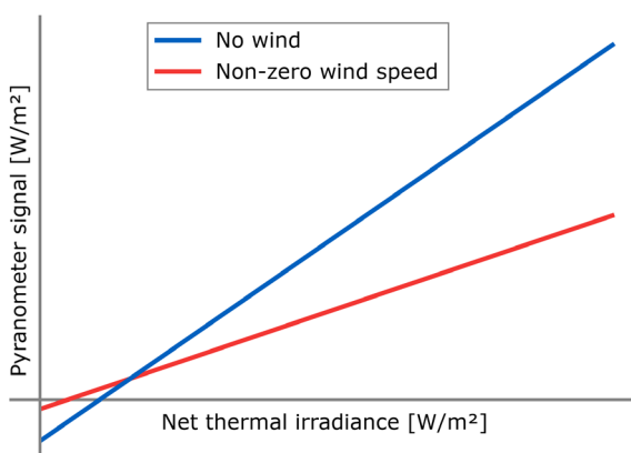
Figure 2 a sketch of the pyranometer response to thermal radiation. The slope is the sensitivity to thermal radiation, any offset is attributed to other factors. Note that the slope will also depend on other factors such as wind speed.
