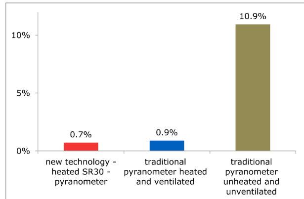
Figure 4 Improving data availability by ventilation: on the vertical axis: unreliable data % of time. On our roof we analysed the data availability with an outdoor camera. We manually marked the moments that the pyranometer was covered with dew or frost. In autumn season with a traditional pyranometer (brown on the right) about 10 % of the time the data was not available. Because this was mainly in the early morning, this 10 % of time represented around 3 % of the total solar energy. With traditional external ventilation, the performance was much better, in blue around 1 %. With an SR30 with internal ventilation, in red, the performance is as good as with external ventilation.
