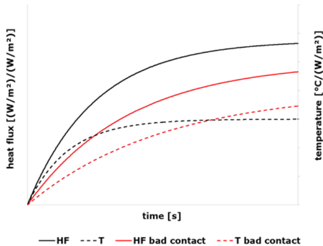
Figure 2.4.1 In situ sensor stability check. Comparison of responses to stepwise heating relative to reference curves. Normalised to heater power (P) and relative to the heat flux and the temperature just before heating. Solid graphs show heat flux, dotted graphs show temperature. The black HF and T signals are the reference curves at good thermal contact. The sensor loses thermal contact, which results in the red responses: slower response times, lower heat flux and higher temperature rise.
