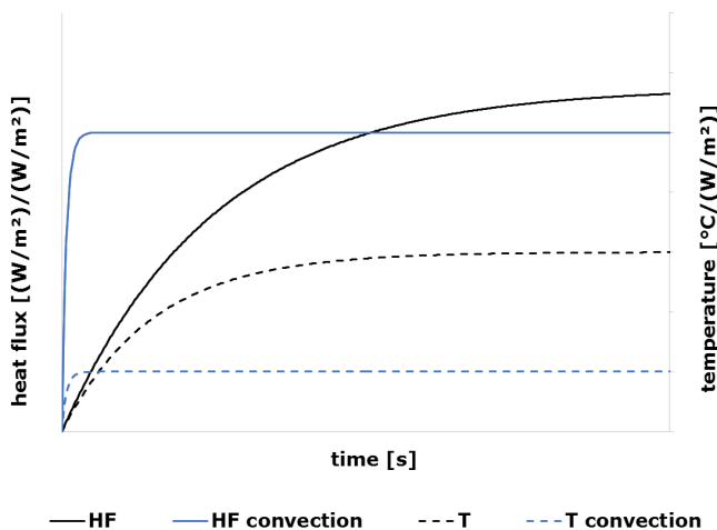
Figure 2.4.2 In situ sensor stability check. Comparison of responses to stepwise heating relative to reference curves. Normalised to heater power (P) and relative to the heat flux and the temperature just before heating. Solid graphs show heat flux, dotted graphs show temperature. The black HF and T signals are the reference curves at zero wind speed. The sensor is exposed to convection, which results in the blue responses: faster response times at lower heat flux and lower temperature rise.
