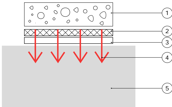
Figure 3 Working with HTR01; a typical stack used for calibration consists of a block of metal (mass > 1 kg), for example aluminium (5), the heat flux sensor (3), the HTR01 (2) and an insulation foam (1). Under these conditions, heat losses through the insulation are negligible. Heat flux flows from hot to cold. Dimensions in \times 10^{-3} m.
