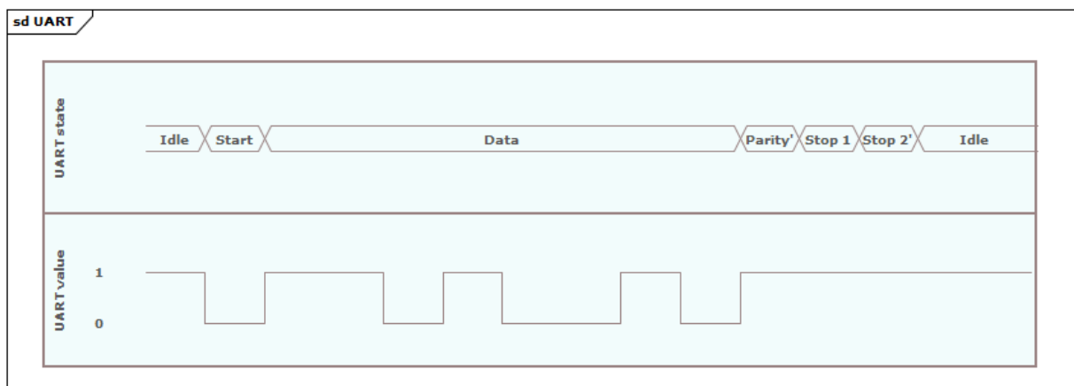
Figure 1.1.1: An example UART frame.
