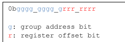
Figure 2.2.1: Register address constructed from group start address and register offset.
