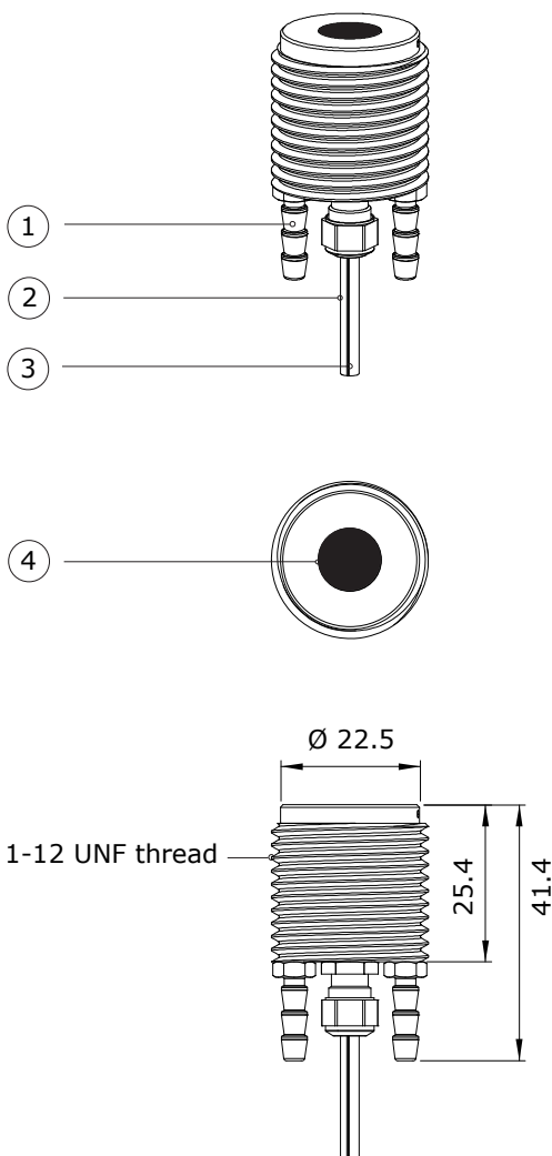
Figure 4 The optional SBG01-T showing its threaded body with optional type T thermocouple. from top to bottom: 3D view, front view, side view. Dimensions in \times 10^{-3} \text{ m} . (1) water cooling tube, outer diameter tubes 4.2 \times 10^{-3} \text{ m} , (2) cable, (3) thermocouple cable, standard cable length is 2 m, (4) thermopile sensor with black coating.
